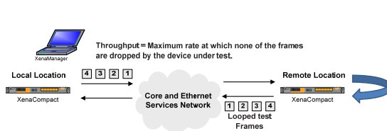
▪ Figure 3 RFC 2544 Throughput Test
