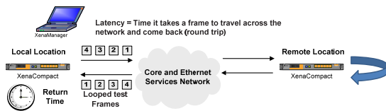
▪ Figure 5 RFC 2544 Latency Test
