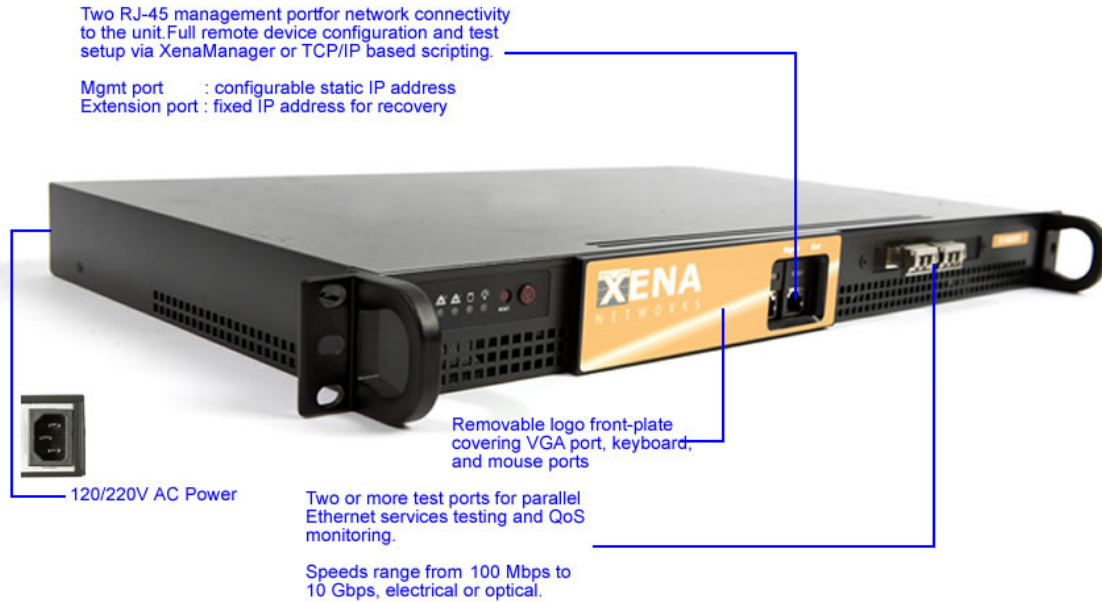
▪ Figure 1 XenaCompact Ethernet Test and Management Interfaces
