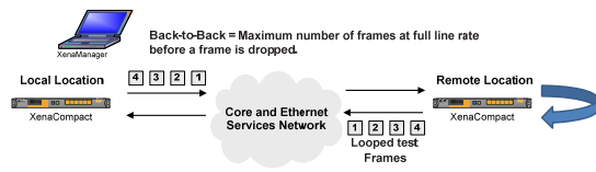
▪ Figure 6 RFC 2544 Back-to-Back Test
