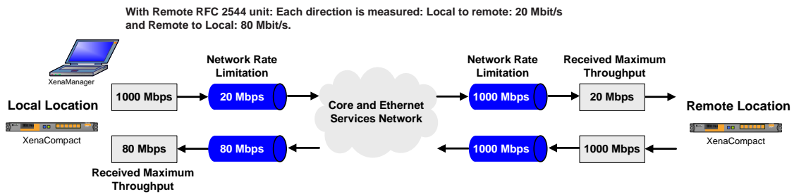
▪ Figure 8 Uni-Directional RFC2544 Testing (Dual Test Set)
