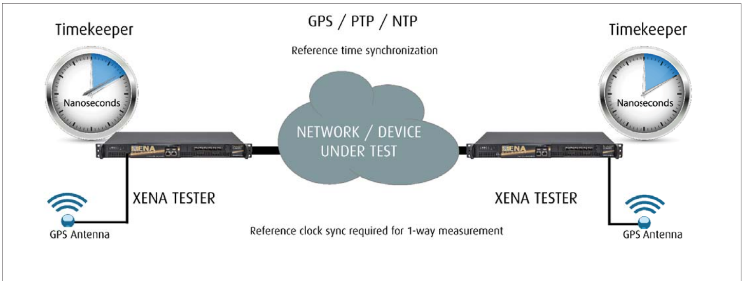
This diagram shows One-Way Latency (OWL) testing over a WAN using Xena TimeSynch .
