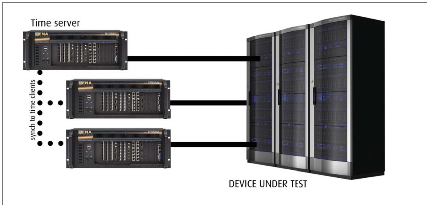
This diagram shows One-Way Latency (OWL) testing over a WAN using Xena TimeSynch .
