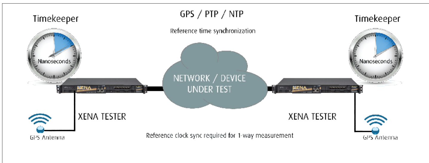
This diagram shows One-Way Latency (OWL) testing over a WAN using ValkyrieTimeSynch .
