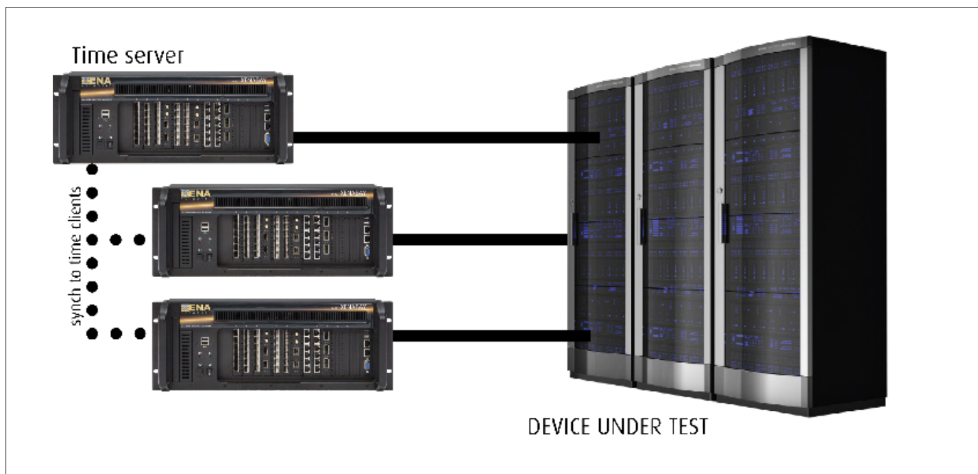
This diagram shows One-Way Latency (OWL) testing over a WAN using ValkyrieTimeSynch .
